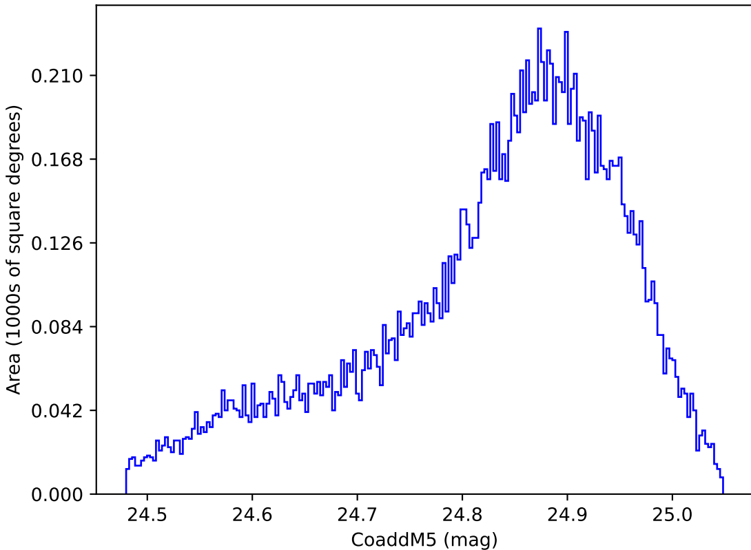
all_long_v3.4_10yrs WFD y band: CoaddM5
