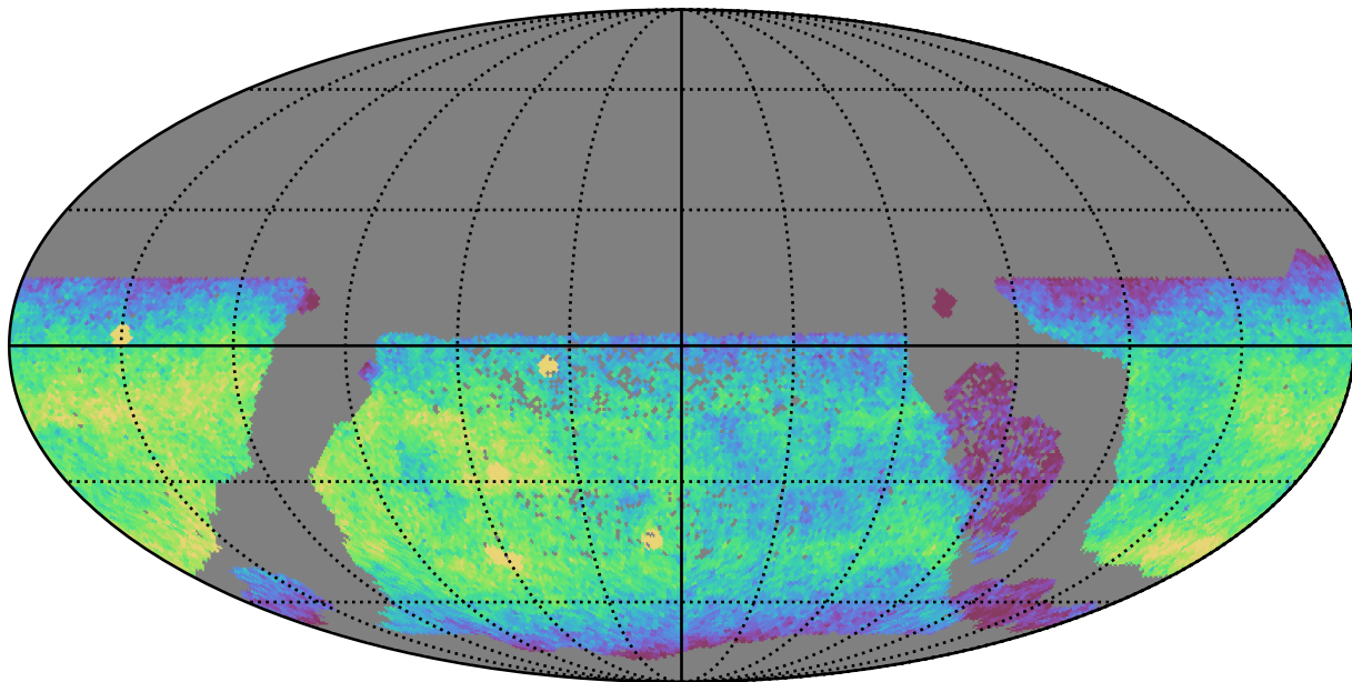
all_long_v3.4_10yrs WFD u band: CoaddM5
