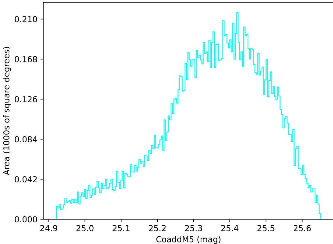
all_long_v3.4_10yrs WFD u band: CoaddM5
