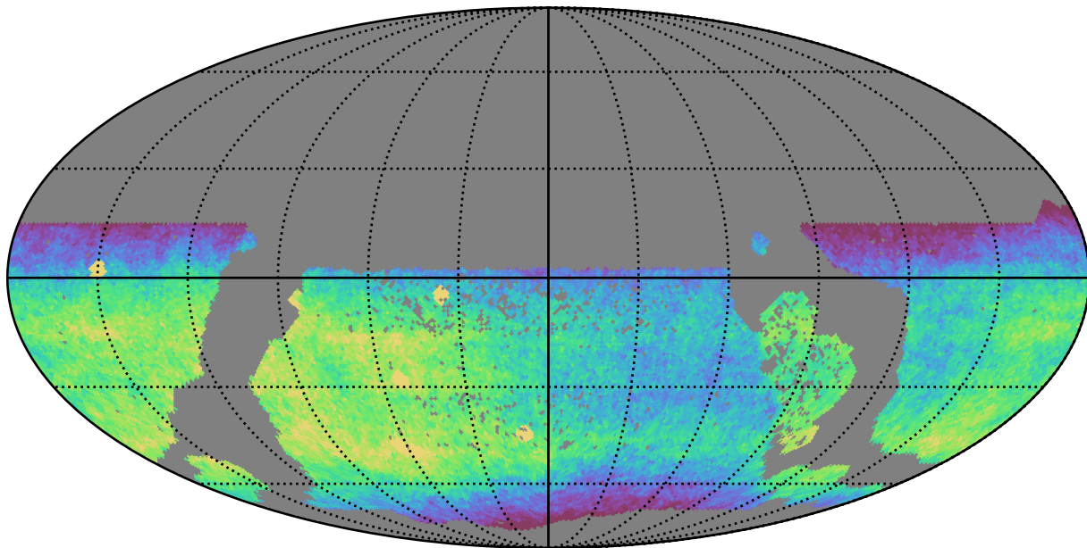
all_long_v3.4_10yrs WFD r band: CoaddM5
