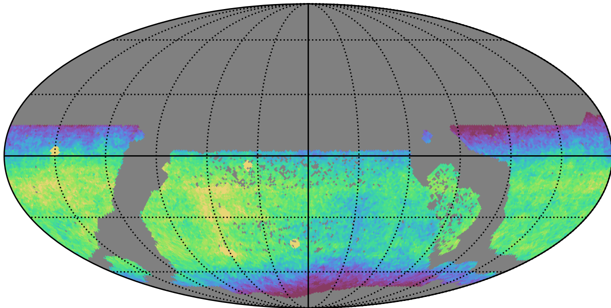
all_long_v3.4_10yrs WFD i band: CoaddM5
