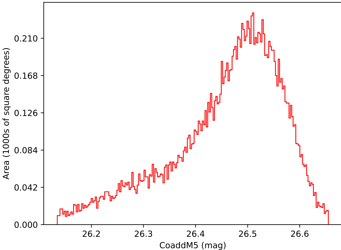
all_long_v3.4_10yrs WFD i band: CoaddM5
