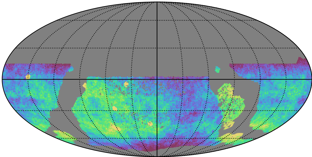
all_long_v3.4_10yrs WFD g band: CoaddM5
