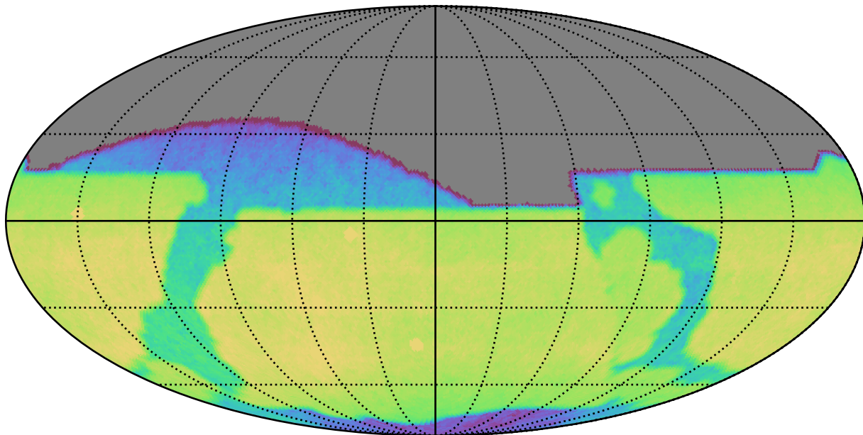
all_long_v3.4_10yrs All sky z band: CoaddM5
