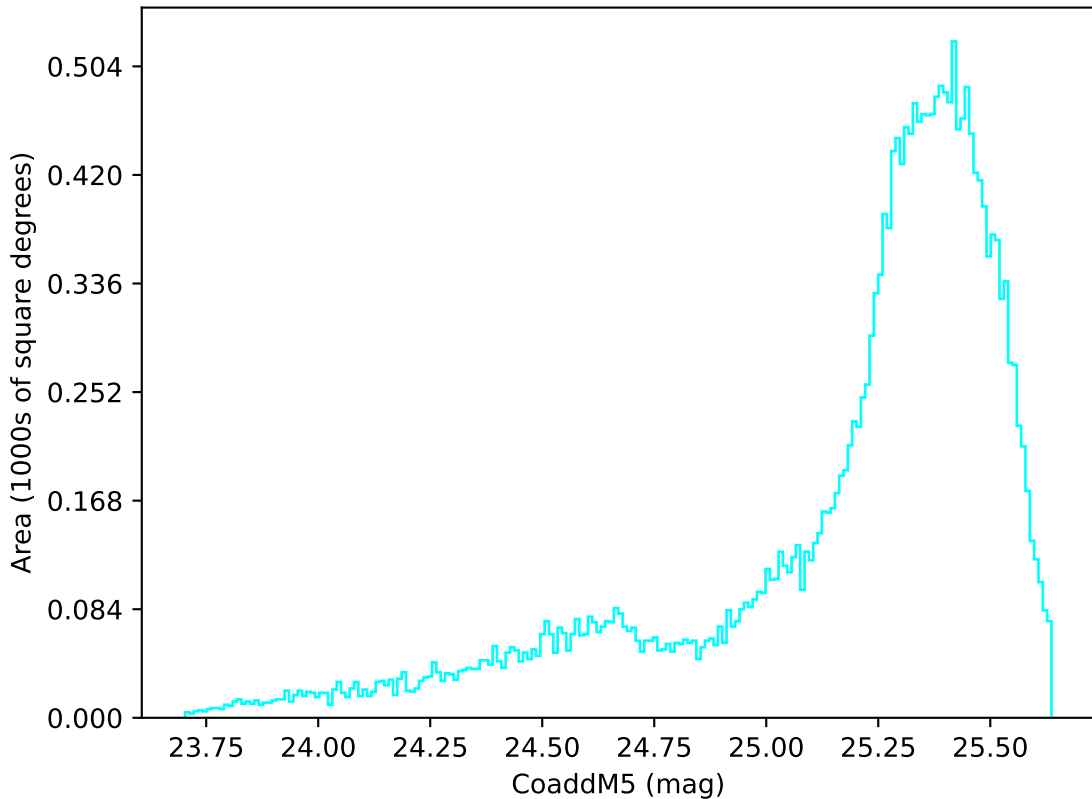
all_long_v3.4_10yrs All sky u band: CoaddM5
