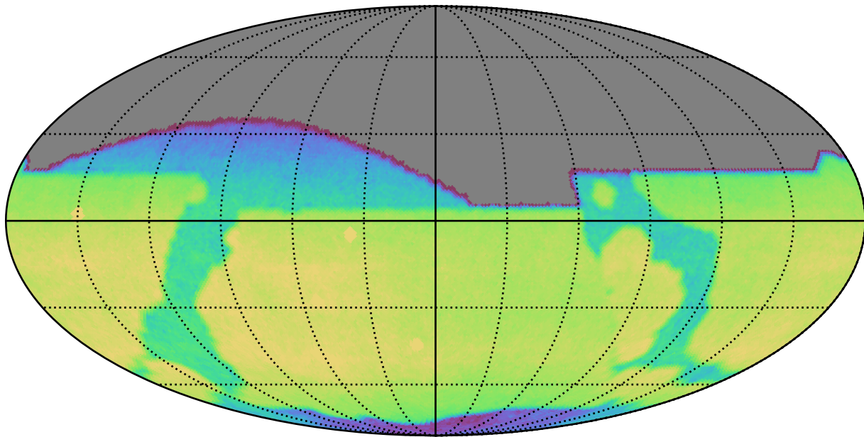
all_long_v3.4_10yrs All sky r band: CoaddM5
