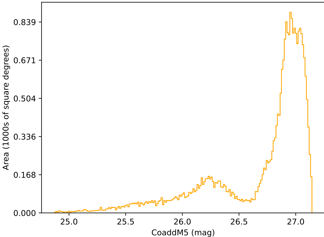
all_long_v3.4_10yrs All sky r band: CoaddM5
