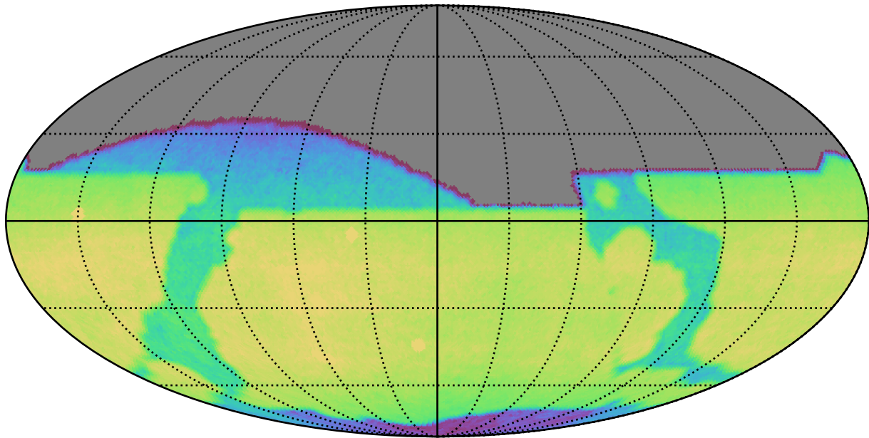
all_long_v3.4_10yrs All sky i band: CoaddM5
