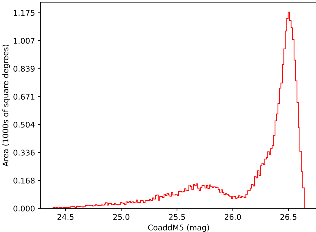
all_long_v3.4_10yrs All sky i band: CoaddM5
