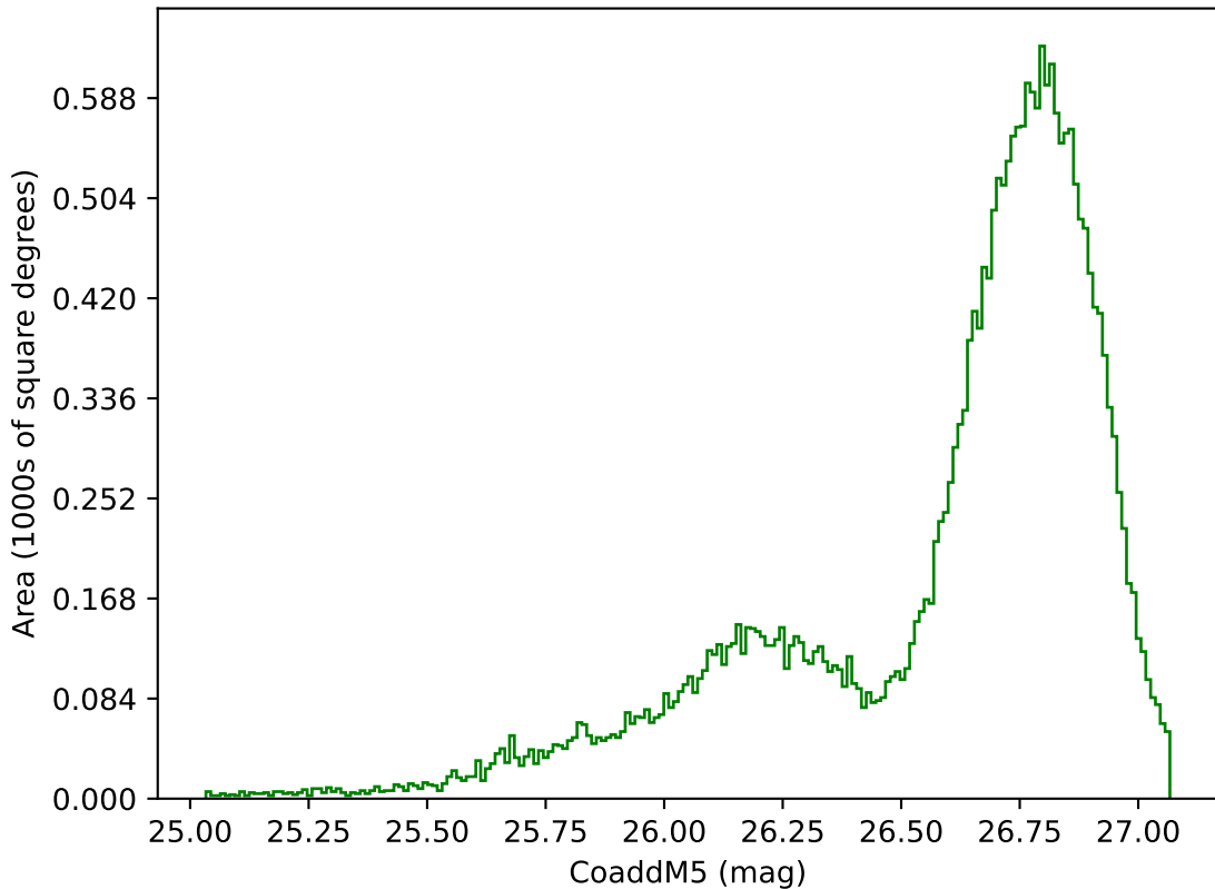
all_long_v3.4_10yrs All sky g band: CoaddM5
