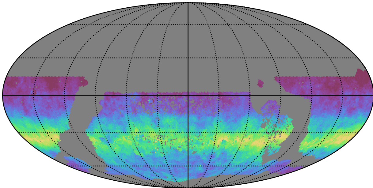
all_long_v3.4_10yrs WFD z band: AngleRms rotSkyPos
