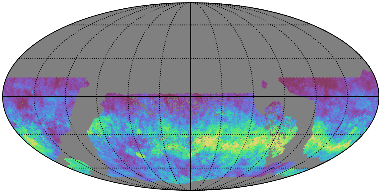
all_long_v3.4_10yrs WFD u band: AngleRms rotSkyPos
