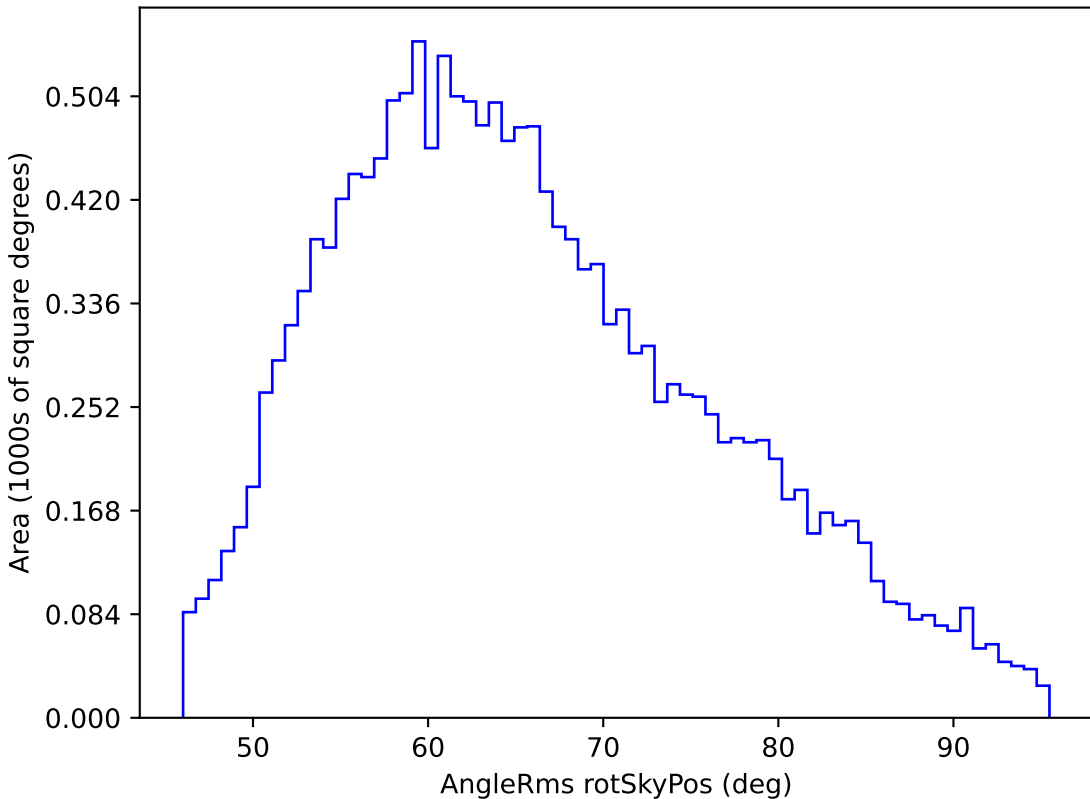
all_long_v3.4_10yrs WFD u band: AngleRms rotSkyPos
