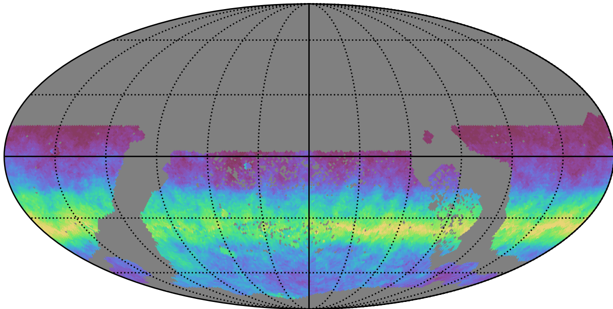
all_long_v3.4_10yrs WFD r band: AngleRms rotSkyPos
