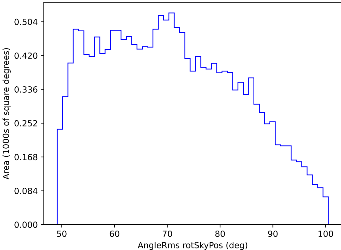
all_long_v3.4_10yrs WFD r band: AngleRms rotSkyPos
