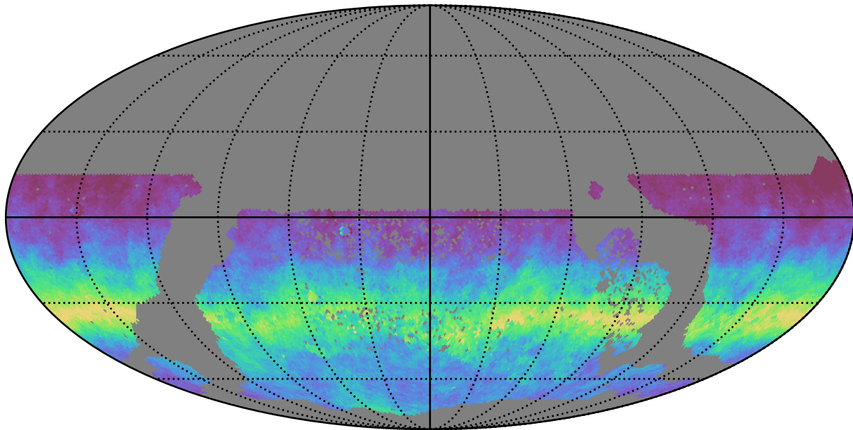
all_long_v3.4_10yrs WFD i band: AngleRms rotSkyPos
