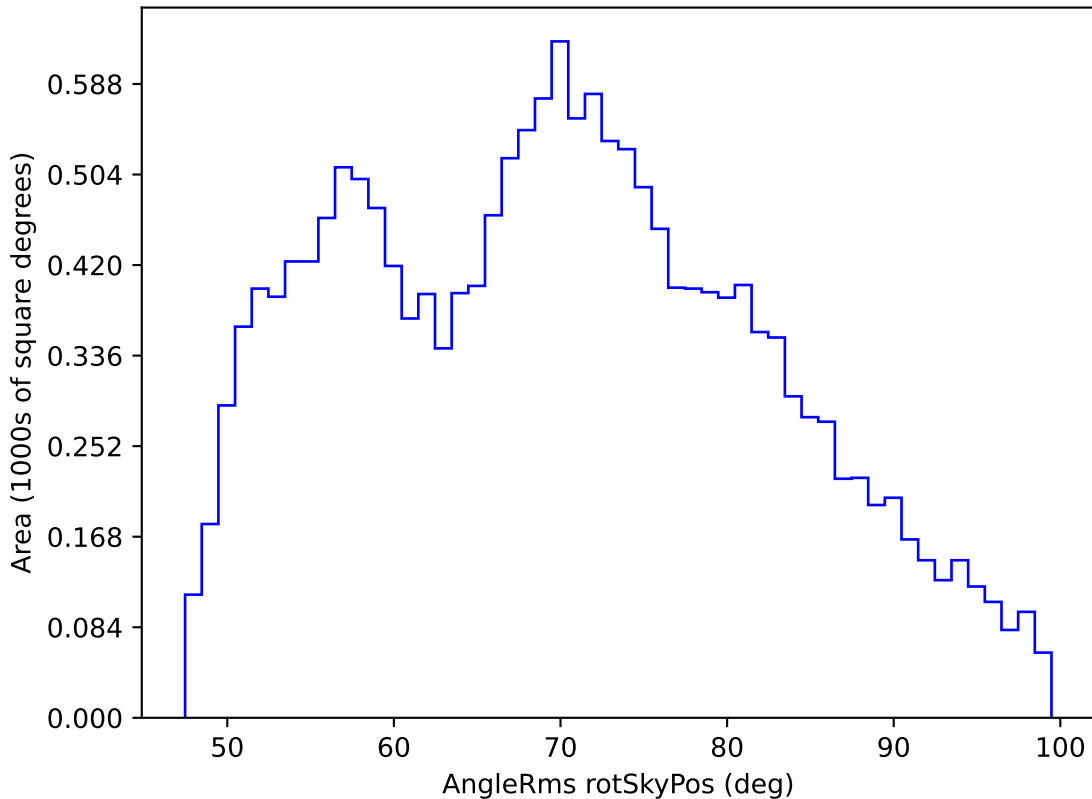
all_long_v3.4_10yrs WFD i band: AngleRms rotSkyPos
