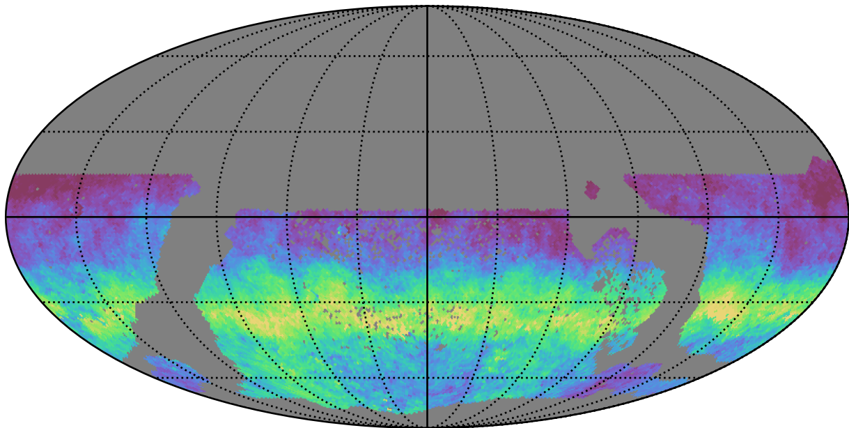
all_long_v3.4_10yrs WFD g band: AngleRms rotSkyPos
