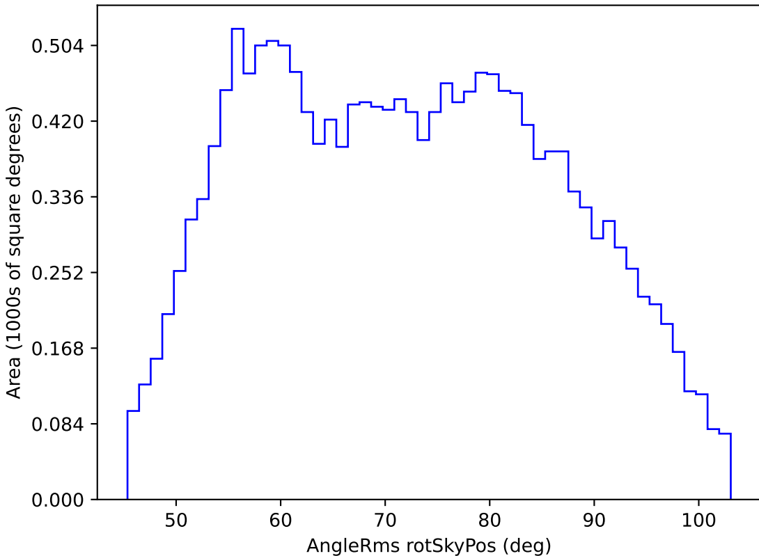
all_long_v3.4_10yrs WFD g band: AngleRms rotSkyPos
