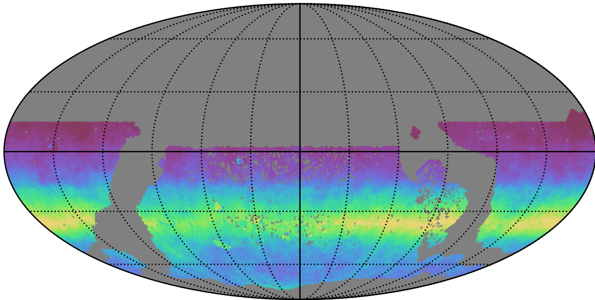
all_long_v3.4_10yrs WFD all bands: AngleRms rotSkyPos
