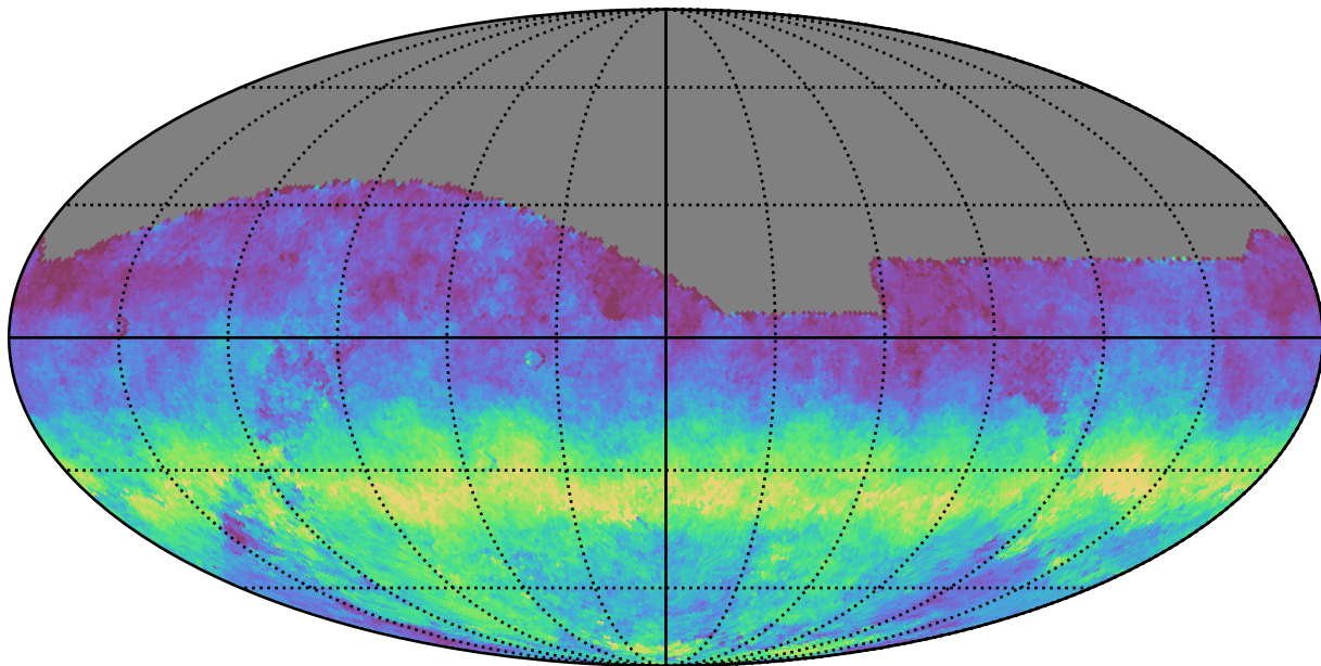
all_long_v3.4_10yrs All sky g band: AngleRms rotSkyPos
