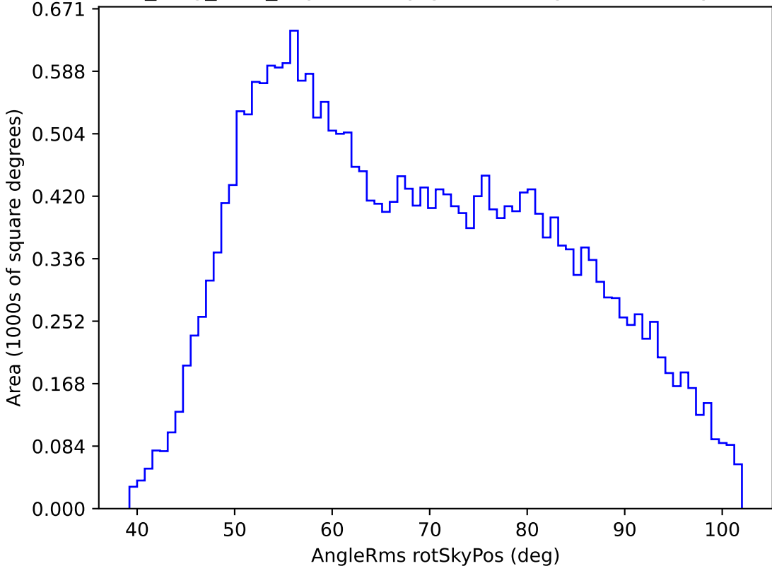
all_long_v3.4_10yrs All sky g band: AngleRms rotSkyPos
