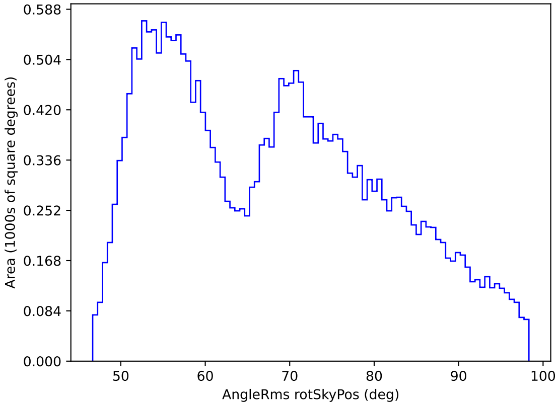
all_long_v3.4_10yrs All sky all bands: AngleRms rotSkyPos
