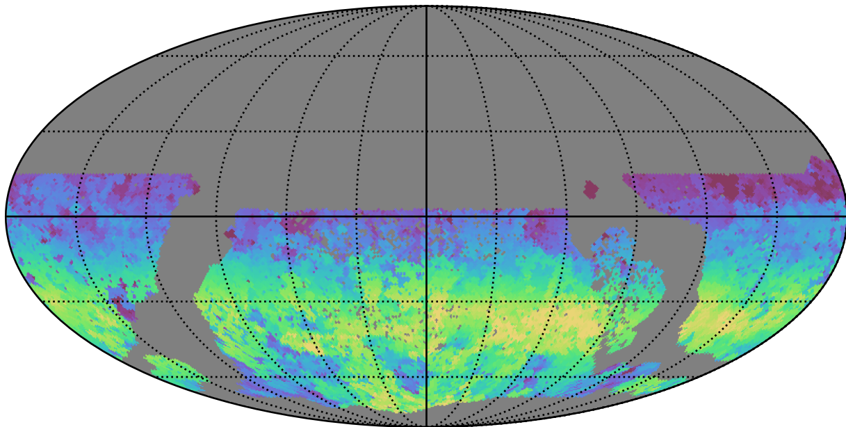
all_long_v3.4_10yrs WFD u band: AngleRange rotSkyPos
