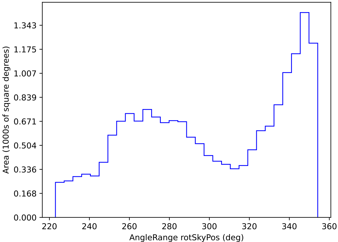
all_long_v3.4_10yrs WFD all bands: AngleRange rotSkyPos
