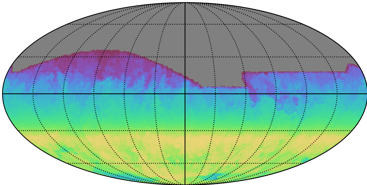
all_long_v3.4_10yrs All sky all bands: AngleRange rotSkyPos
