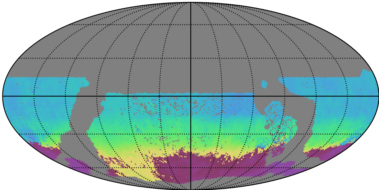
all_long_v3.4_10yrs WFD z band: AngleMean rotSkyPos
