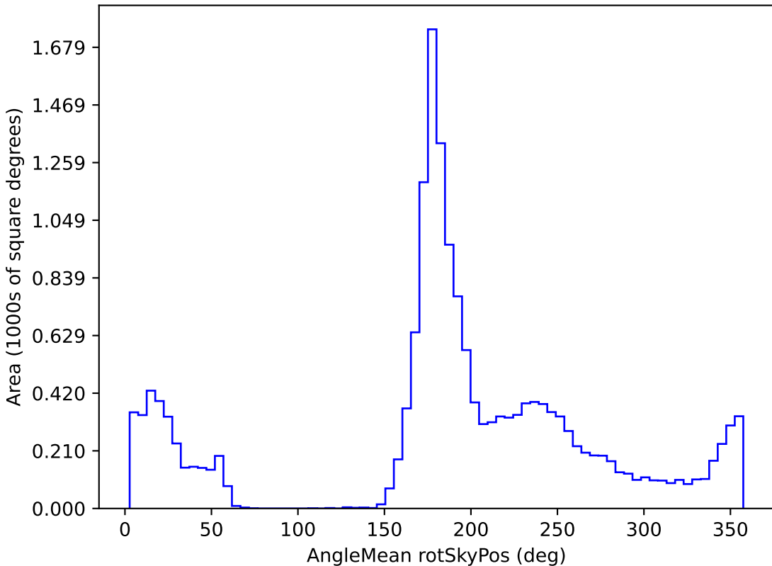
all_long_v3.4_10yrs WFD z band: AngleMean rotSkyPos
