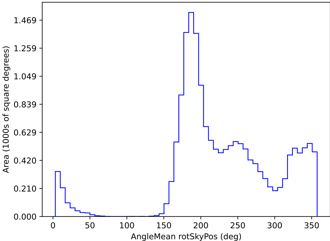
all_long_v3.4_10yrs WFD u band: AngleMean rotSkyPos
