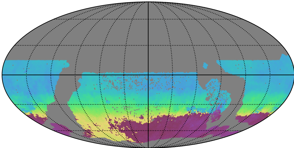
all_long_v3.4_10yrs WFD r band: AngleMean rotSkyPos
