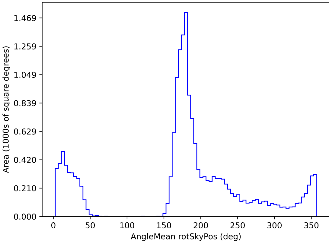
all_long_v3.4_10yrs WFD r band: AngleMean rotSkyPos
