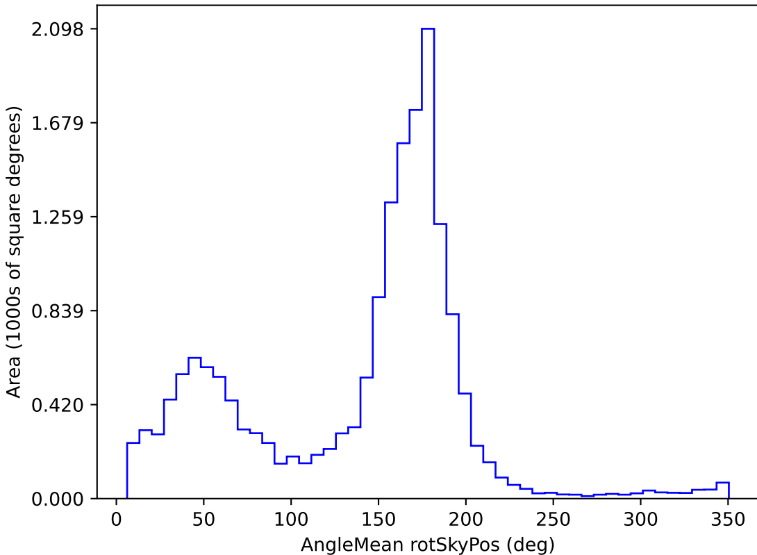
all_long_v3.4_10yrs WFD g band: AngleMean rotSkyPos
