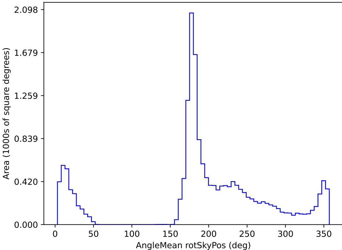
all_long_v3.4_10yrs WFD all bands: AngleMean rotSkyPos
