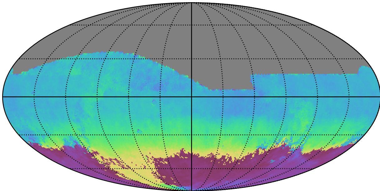
all_long_v3.4_10yrs All sky z band: AngleMean rotSkyPos
