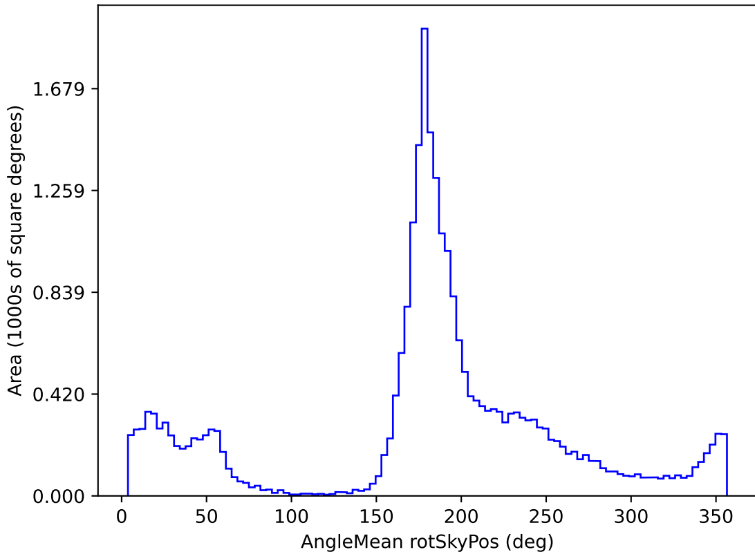
all_long_v3.4_10yrs All sky z band: AngleMean rotSkyPos
