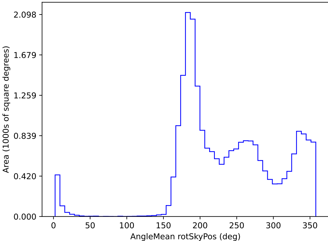
all_long_v3.4_10yrs All sky y band: AngleMean rotSkyPos
