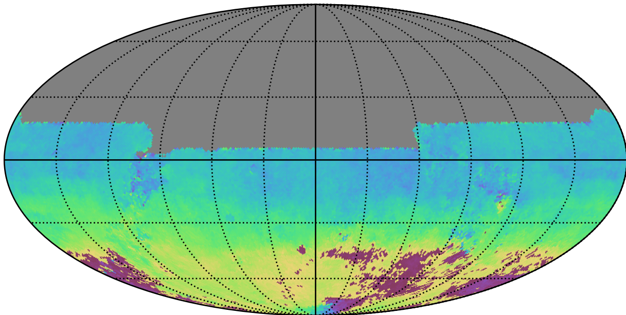
all_long_v3.4_10yrs All sky u band: AngleMean rotSkyPos
