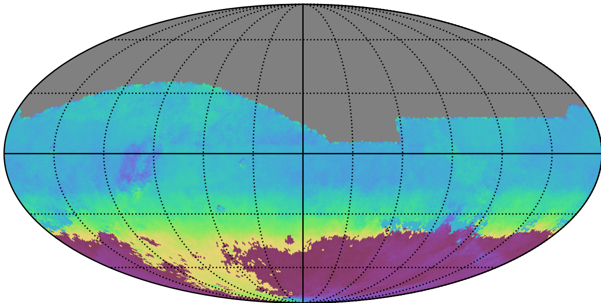
all_long_v3.4_10yrs All sky r band: AngleMean rotSkyPos
