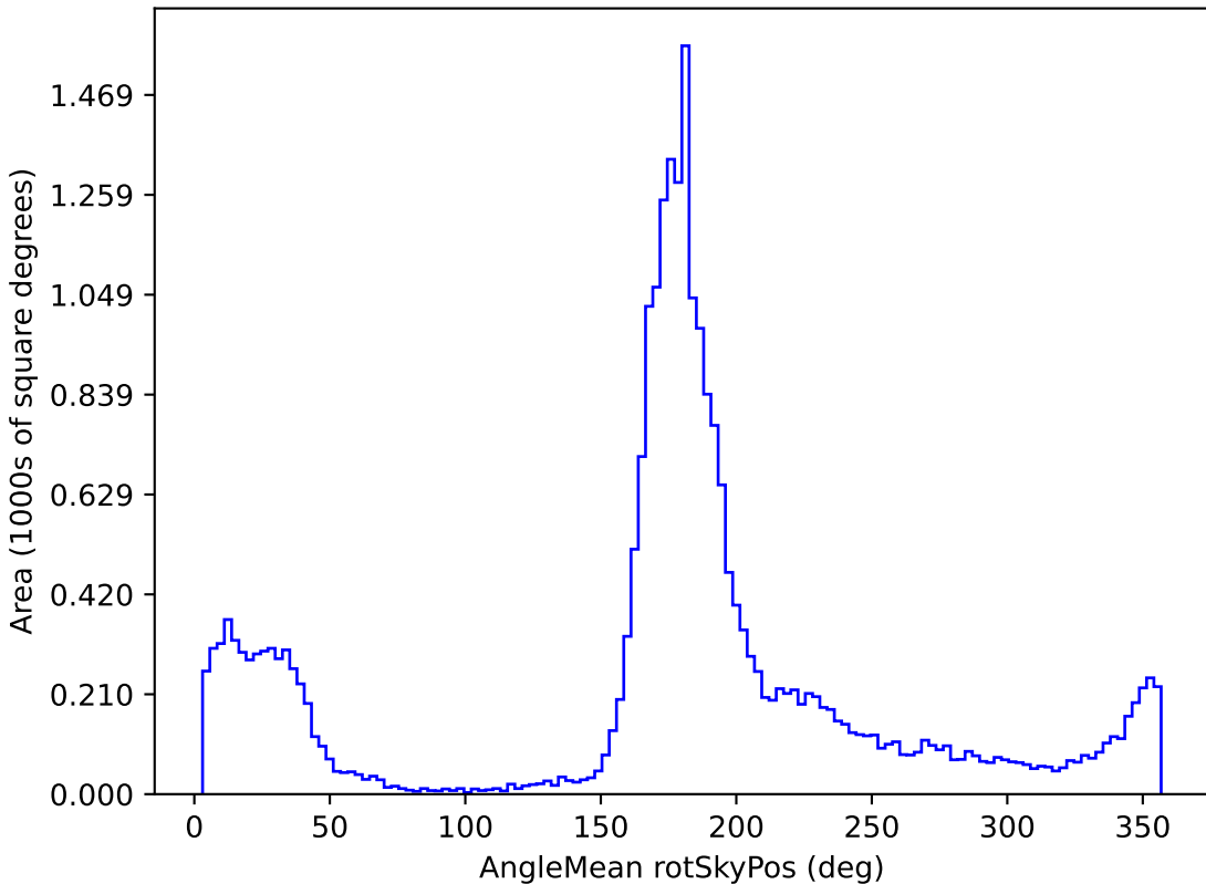
all_long_v3.4_10yrs All sky r band: AngleMean rotSkyPos
