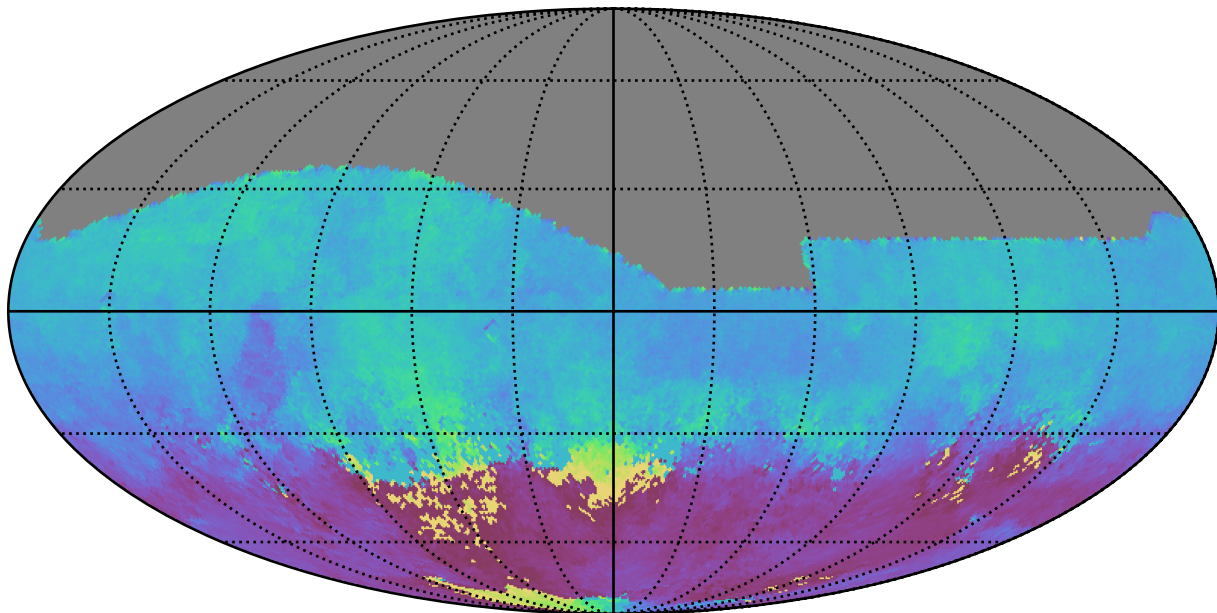
all_long_v3.4_10yrs All sky g band: AngleMean rotSkyPos
