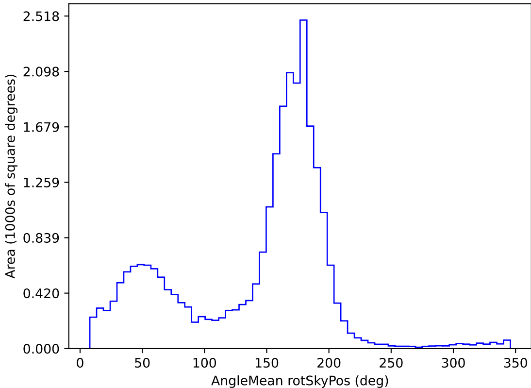
all_long_v3.4_10yrs All sky g band: AngleMean rotSkyPos
