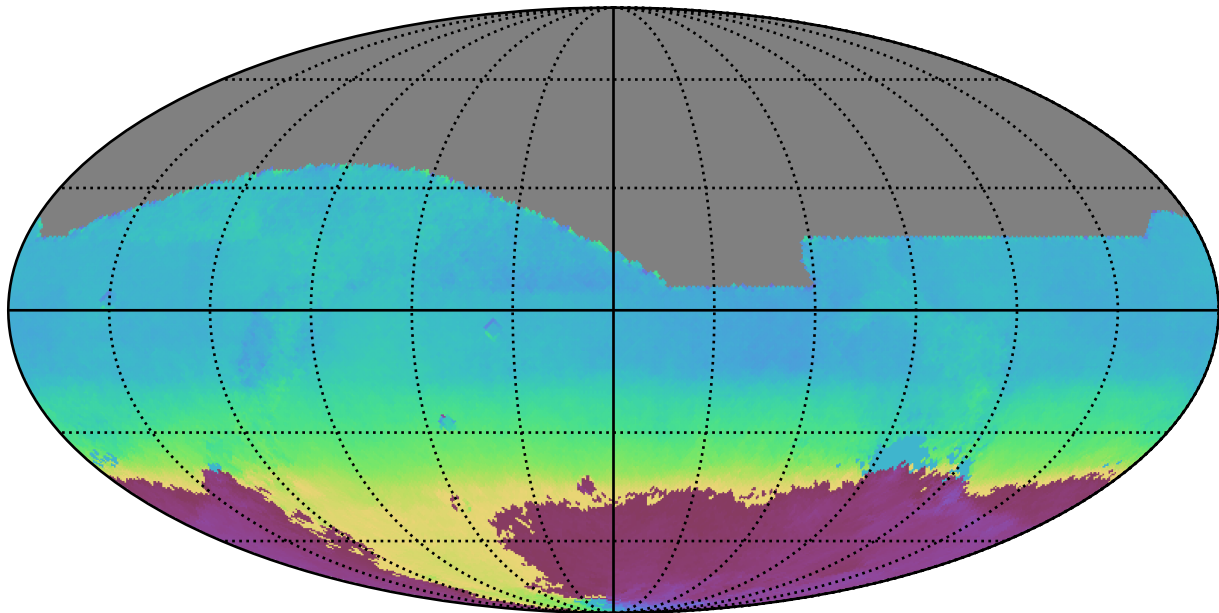
all_long_v3.4_10yrs All sky all bands: AngleMean rotSkyPos
