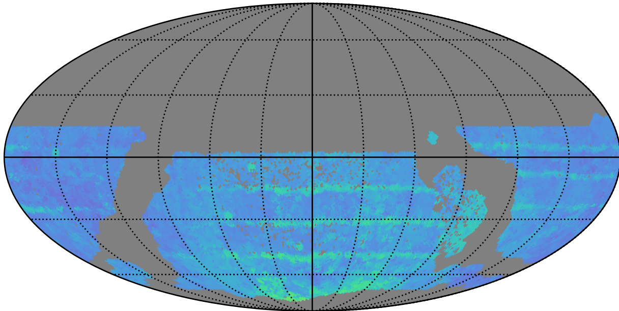
all_long_v3.4_10yrs WFD z band: 80thPercentile Season Length
