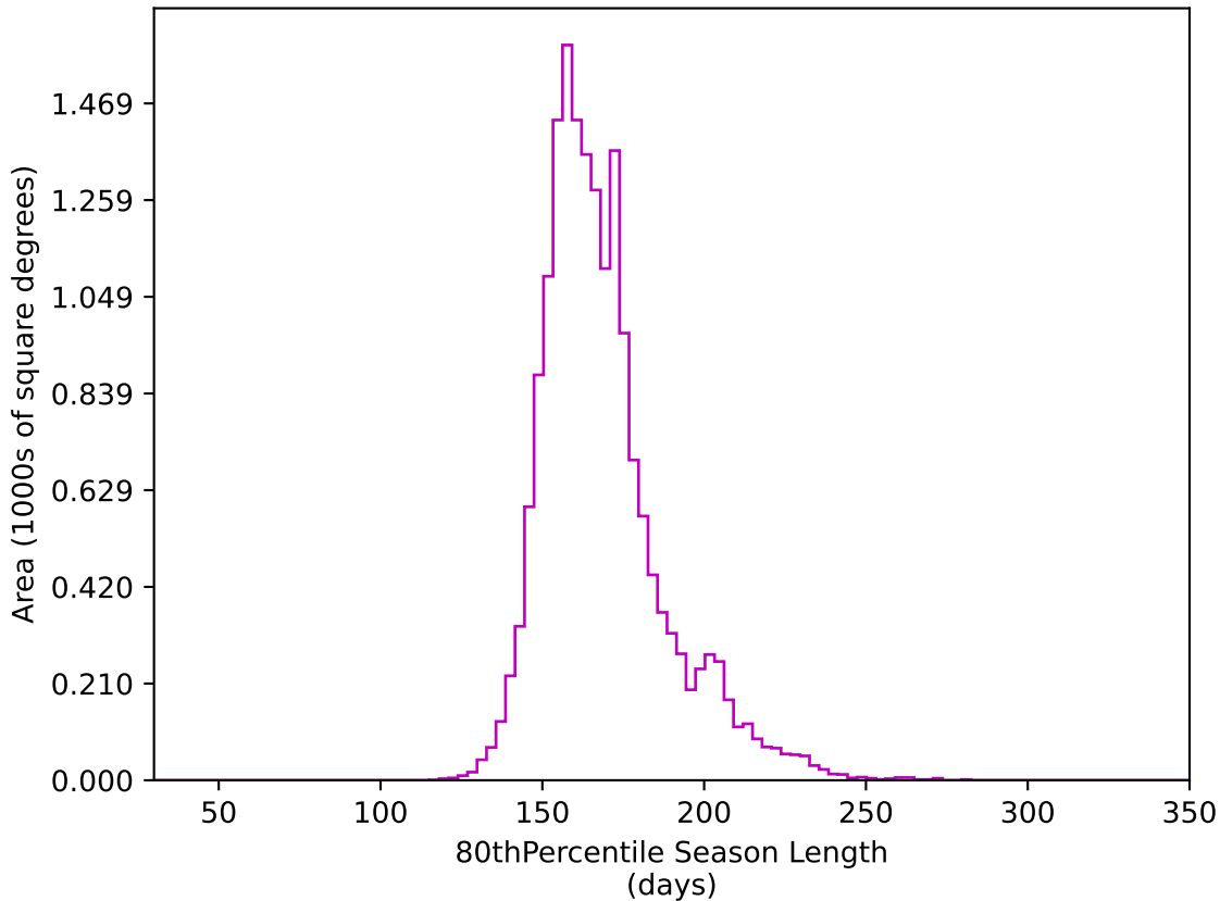
all_long_v3.4_10yrs WFD z band: 80thPercentile Season Length
