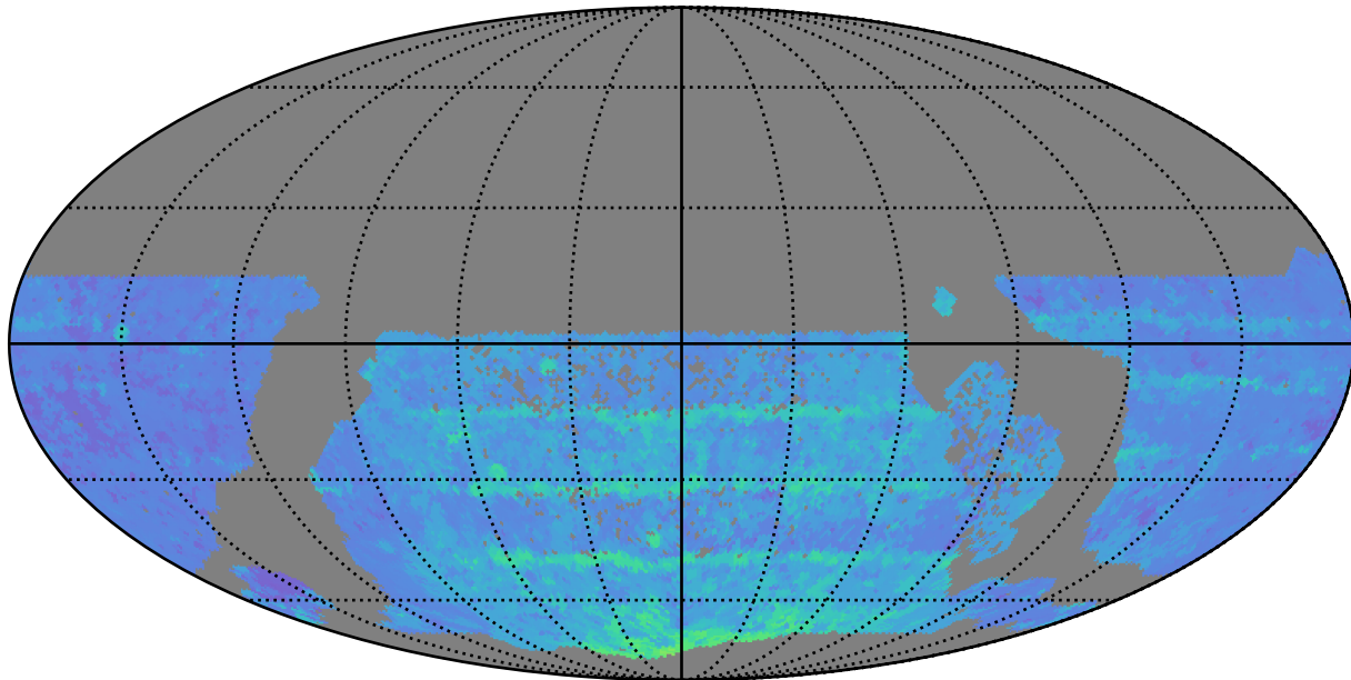
all_long_v3.4_10yrs WFD y band: 80thPercentile Season Length
