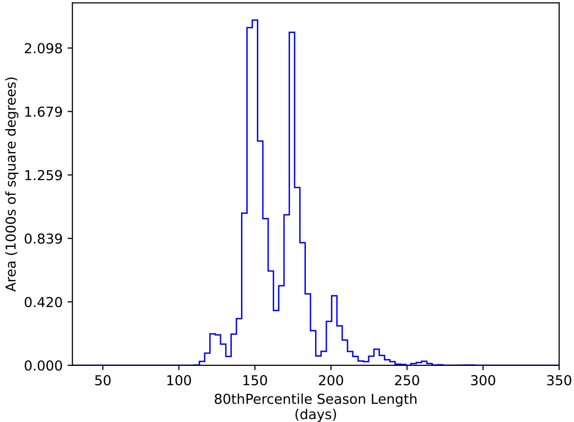
all_long_v3.4_10yrs WFD y band: 80thPercentile Season Length
